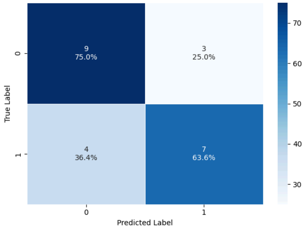
Confusion Matrix: k-NN (k-Nearest Neighbors) Algorithm
