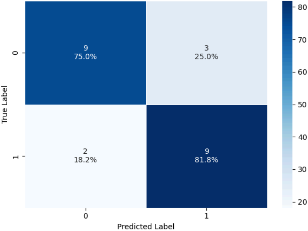
Confusion Matrix: Base Logistic Regression Model
