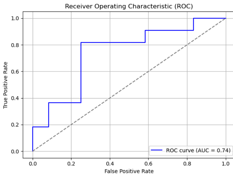
ROC Curve: Base Logistic Regression Model
