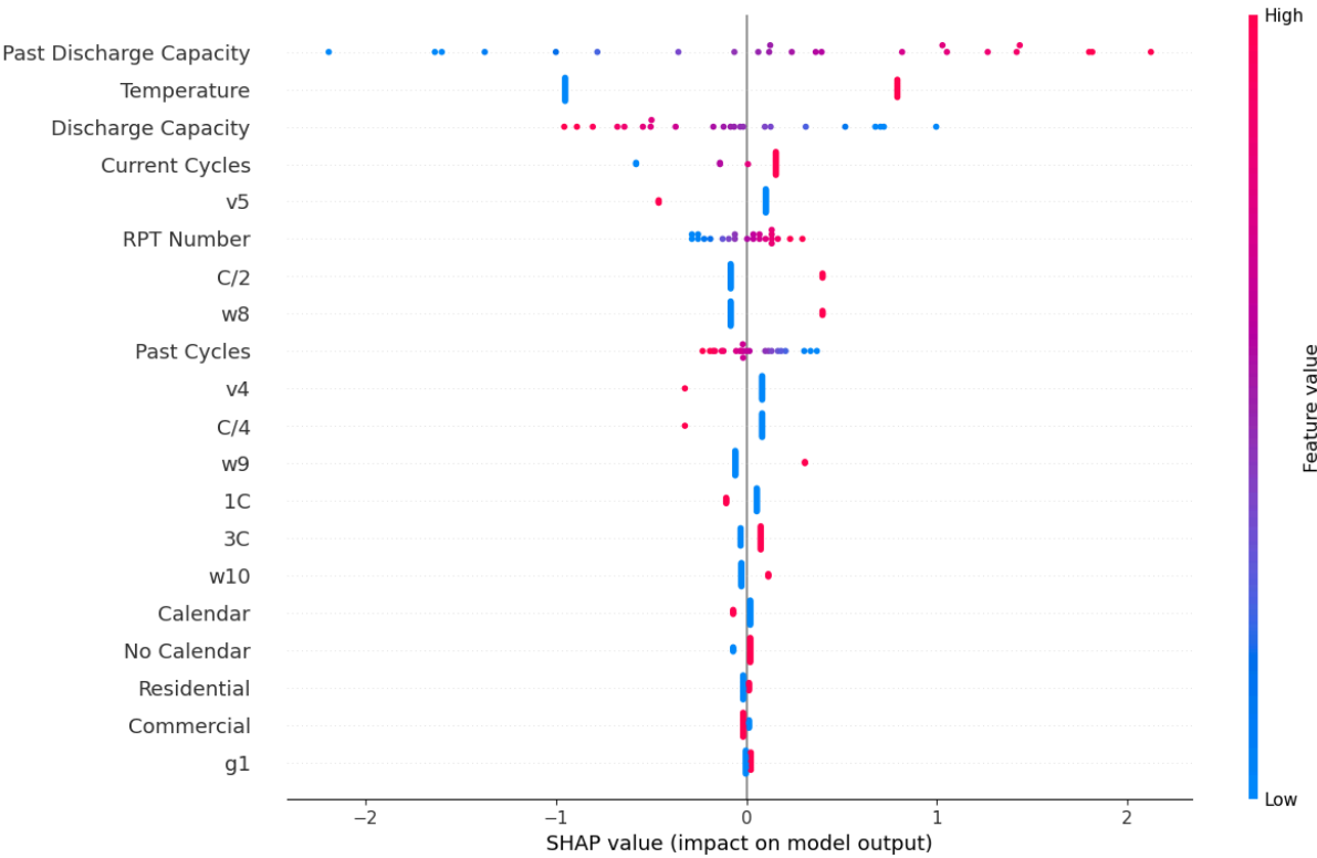
SHAP Beeswarm Plot: Manual Removal Regression
